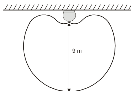
glass break detector working range diagram
